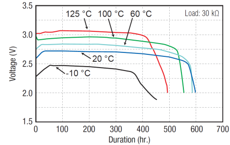
■ Discharge temperature characteristics(e.g. BR1225A)
