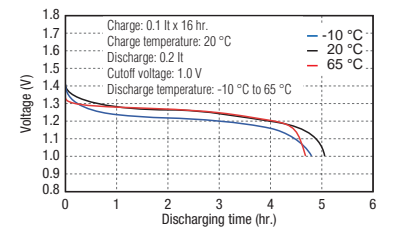
■ Example discharge characteristics
