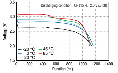
Discharge temperature characteristics (Example: CR2032A)
