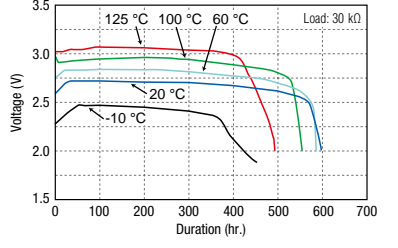
Discharge temperature characteristics (Example: BR1225A)
